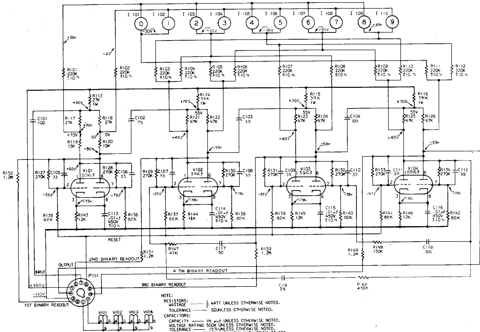
FIGURE 8. MODEL 775 SCHEMATIC DIAGRAM.
